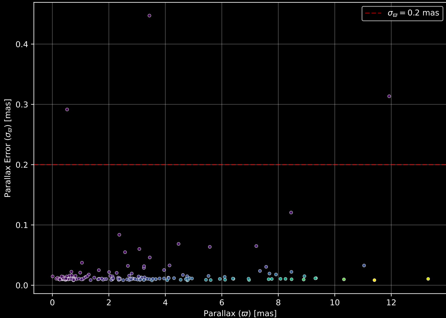
APOGEE DR17 Field: [267-22-O_TESS] Parallax Quality (n= 170)
