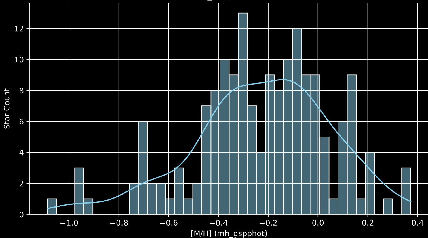
APOGEE DR17 Field: [267-22-O_TESS [M/H] (mh_gspphot) (n= 169)
