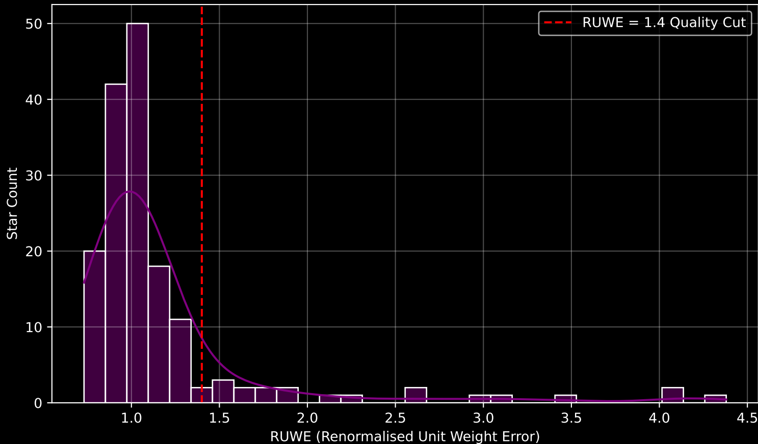
GAPOGEE DR17 Field [267-22-O_TESS] RUWE Distribution (n= 162)
