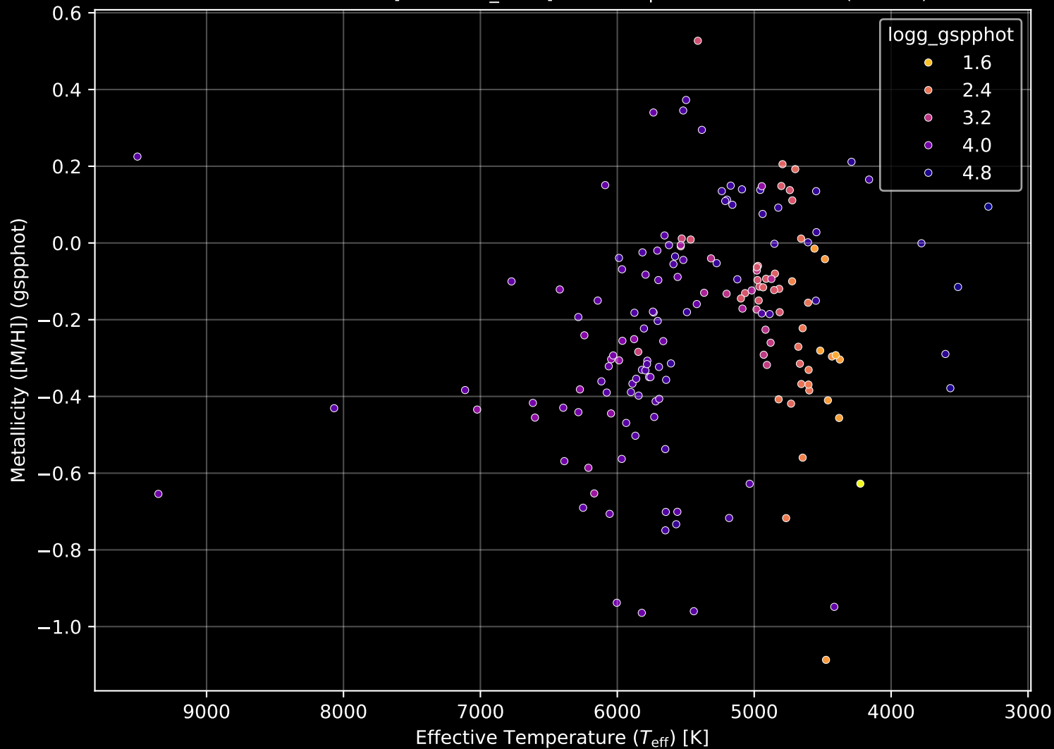
APOGEE DR17 Field: [267-22-O_TESS] Stellar Population Parameters (n= 170)
