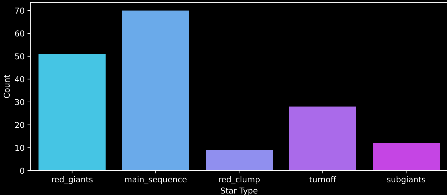
APOGEE DR17 Field: [267-22-O_TESS] Count plot of Star Type
