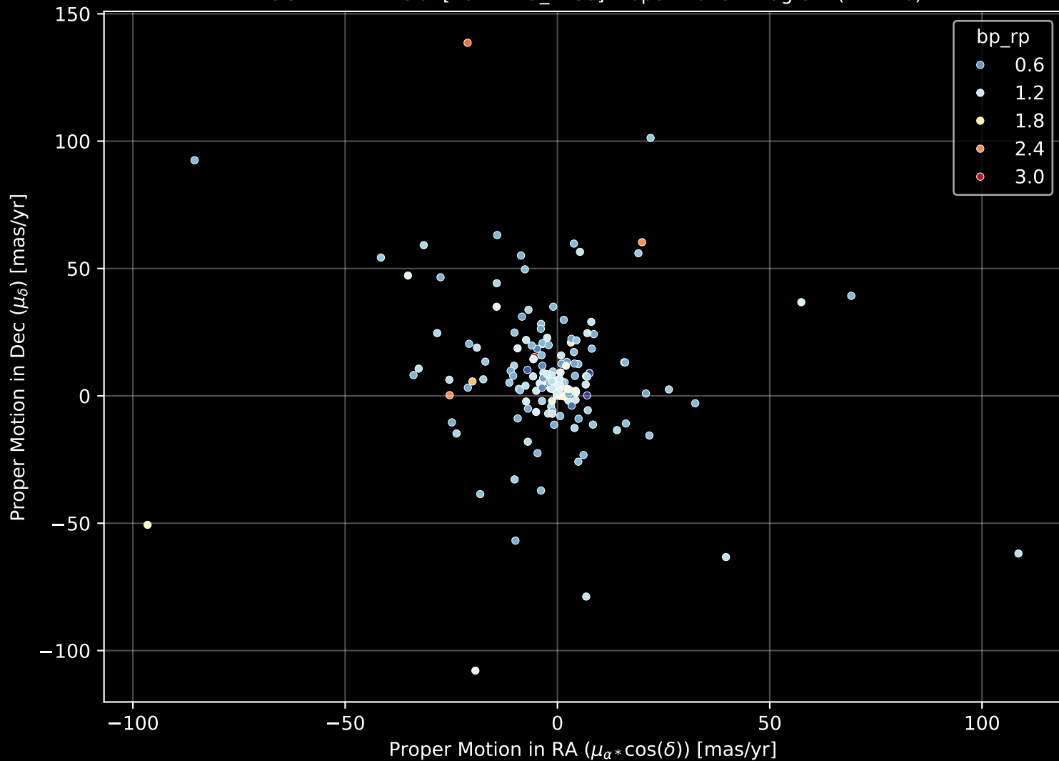
APOGEE DR17 Field: [267-22-O_TESS] Proper Motion Diagram (n= 170)
