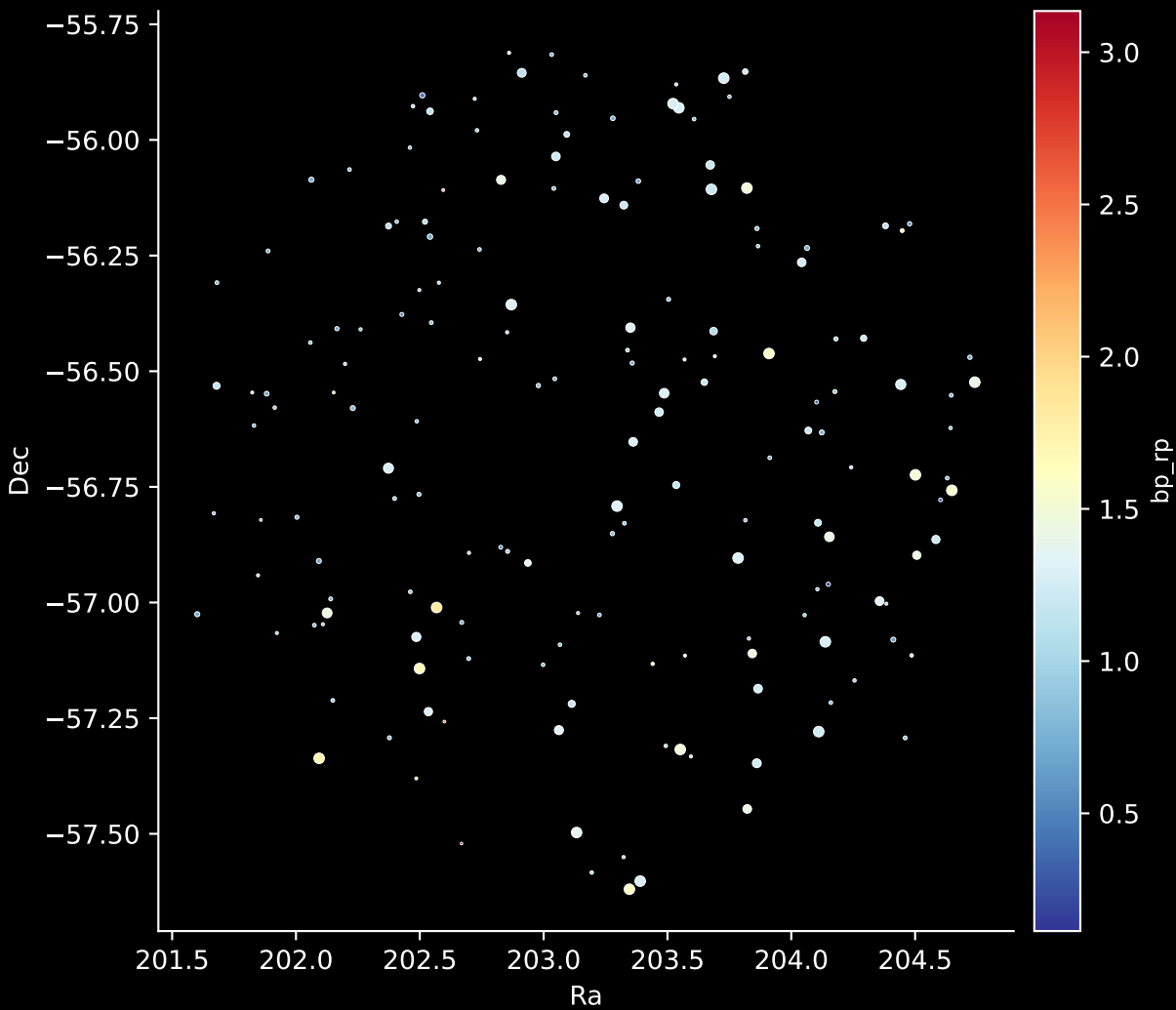
APOGEE DR17 Field: [267-22-O_TESS] Stars: 170
